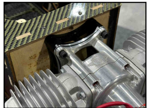
DA-120 mounted with the Apex/Dualsky engine mount
