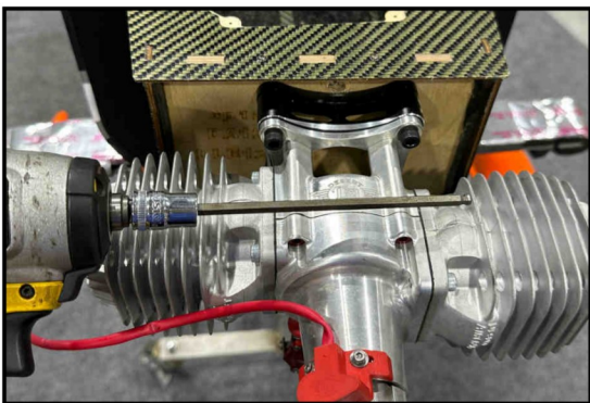
You may use an impact driver for engine installation. This is safe as long as an extension is used.
