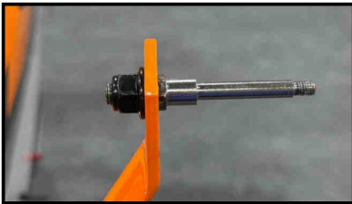
Align the axle so that the hex portion is vertical. This orientation ensures the wheel pant can be installed correctly.
