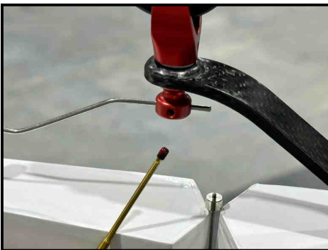
Be sure to install the flat portion of the tiller wire into the tailwheel swivel mount. Apply Loctite to the set screw before tightening.
