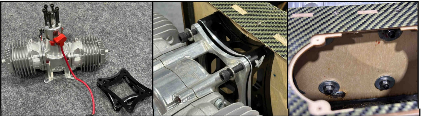
Install fender washers behind the firewall, between the firewall and the locknuts.
