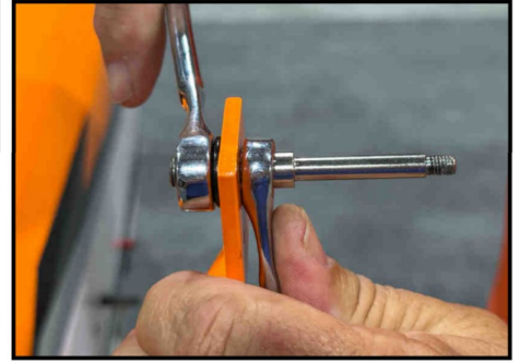
Tighten the axle locknut using two wrenches: one on the locknut and the other on the hex portion of the axle to prevent the axle from turning.
