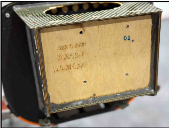
The Slick features pre-drilled mounting holes for the most popular engine options in the 120cc class. The Desert Aircraft 120cc engine will be shown for reference.
